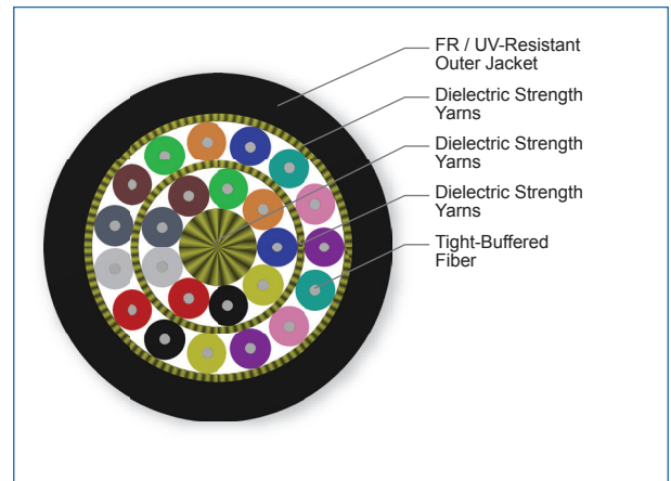
Cross Section of Part Number: 024T8F-31131-29
