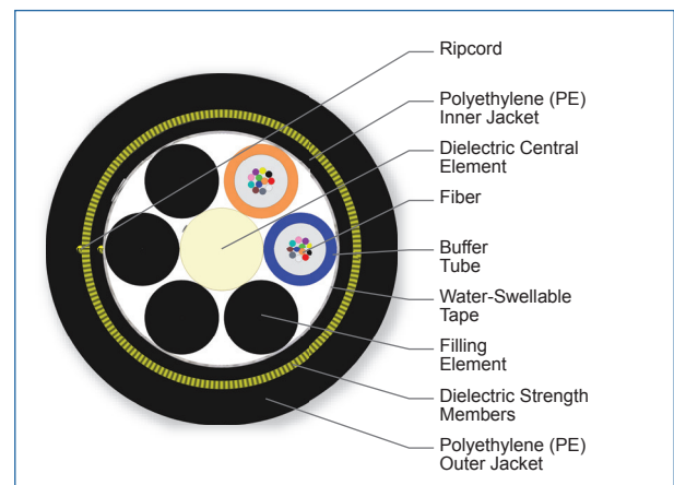
Cross Section of Part Number: 024TAE-T4231A20
