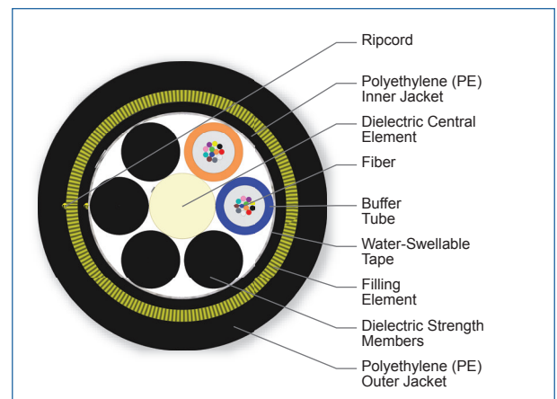
Cross Section of Part Number: 024TAE-T4531A20
