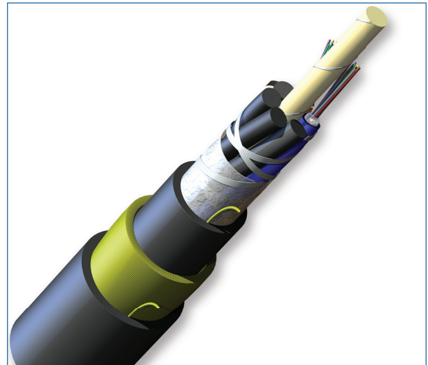
Part Number: 024TAE-T4A31A20
