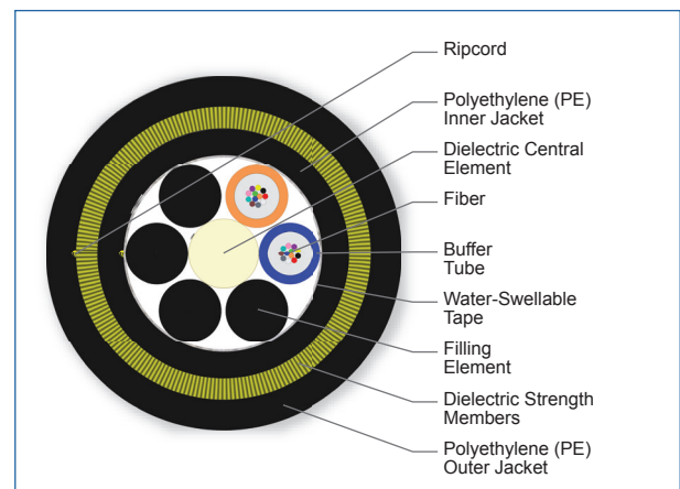
Cross Section of Part Number: 024TAE-T4A31A20
