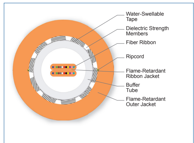
Cross Section of Part Number: 024TC8-94131-20
