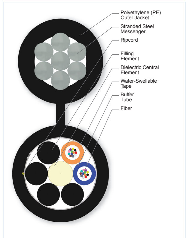
Cross Section of Part Number: 024TUA-T4131D20
