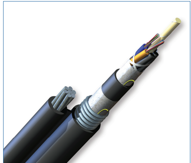
Part Number: 024TUB-T4131D20
