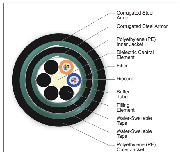
Cross Section of Part Number: 024TUD-T4131A20
