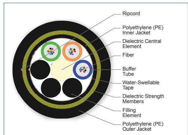
Cross Section of Part Number: 036EAE-T4501A20
