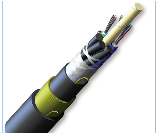
Part Number: 036EAE-T4501A20
