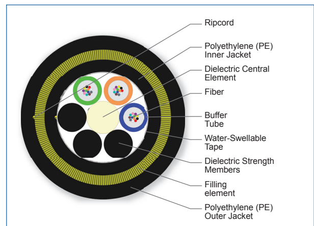
Cross Section of Part Number: 036EAE-T4A01A20
