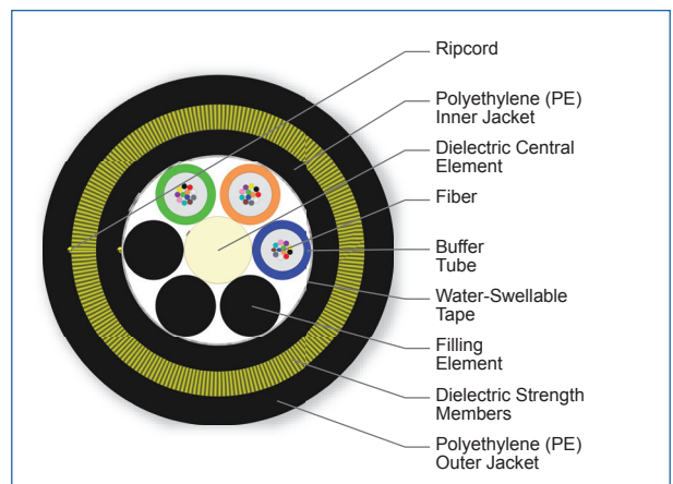
Cross Section of Part Number: 036EAE-T4C01A20
