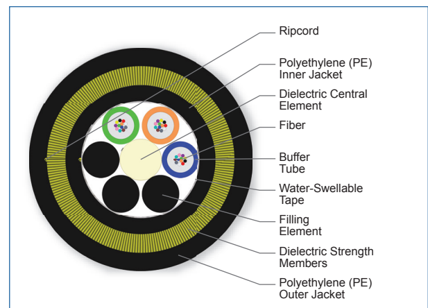
Cross Section of Part Number: 036EAE-T4E01A20
