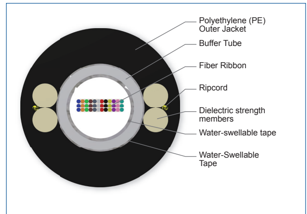
Cross Section of Part Number: 036EC4-14100D53
