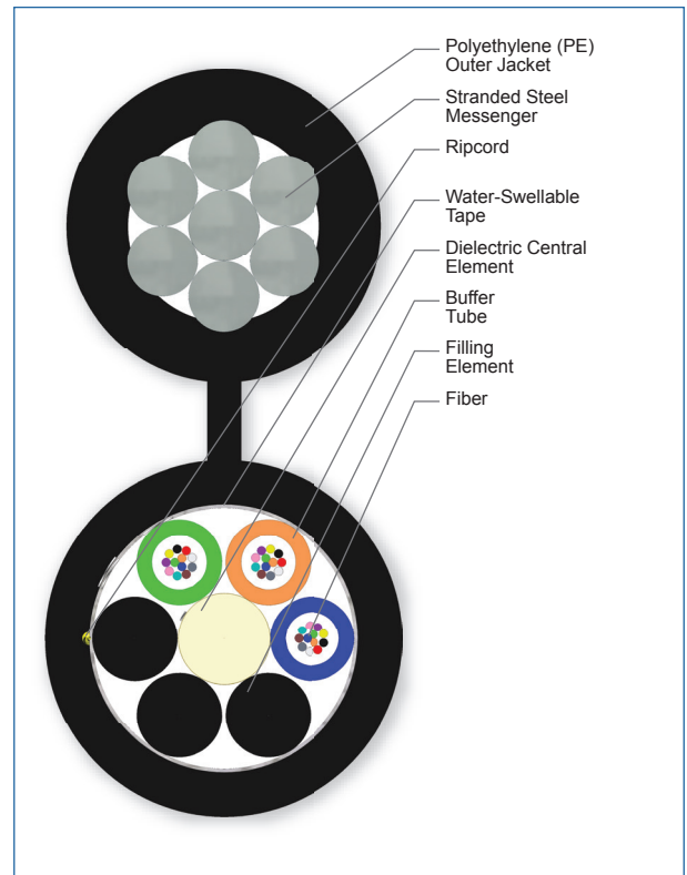
Cross Section of Part Number: 036EUA-T4101D20
