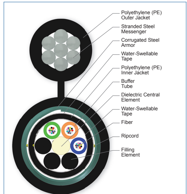
Cross Section of Part Number: 036EUB-T4101D20
