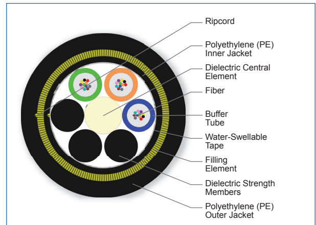
Cross Section of Part Number: 036KAE-T4530A20
