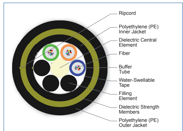
Cross Section of Part Number: 036KAE-T4A30A20
