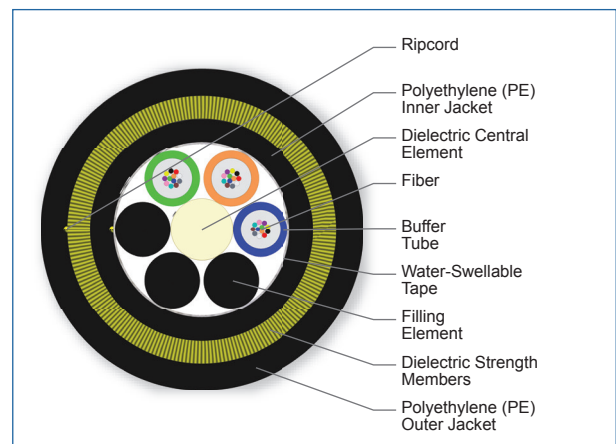
Cross Section of Part Number: 036KAE-T4C30A20
