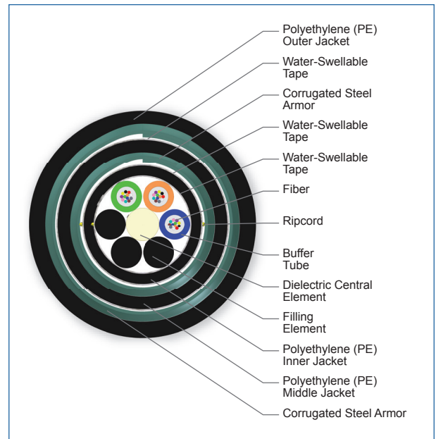
Cross Section of Part Number: 036KU6-T4130A20
