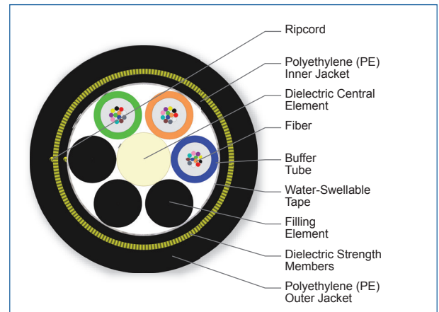
Cross Section of Part Number: 036TAE-T4231A20
