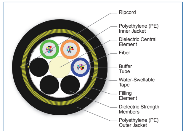
Cross Section of Part Number: 036TAE-T4531A20
