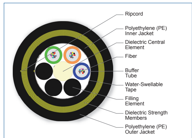
Cross Section of Part Number: 036TAE-T4A31A20
