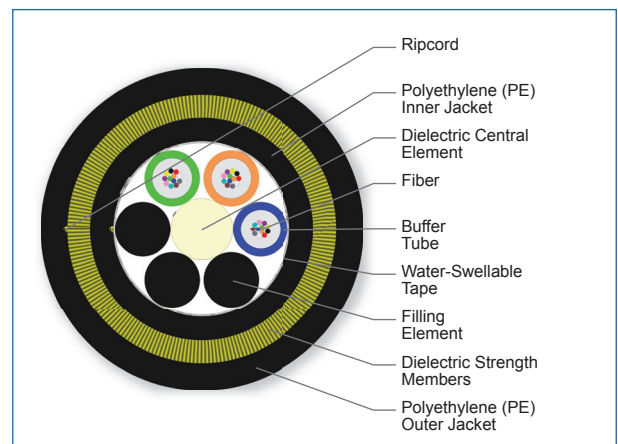
Cross Section of Part Number: 036TAE-T4C31A20
