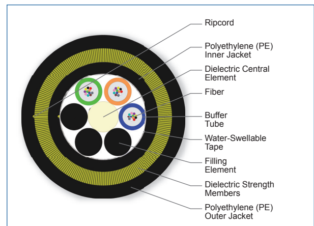
Cross Section of Part Number: 036TAE-T4E31A20
