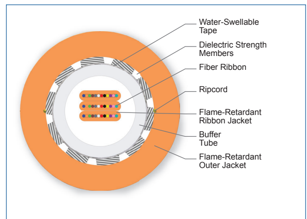
Cross Section of Part Number: 036TC8-94131-20
