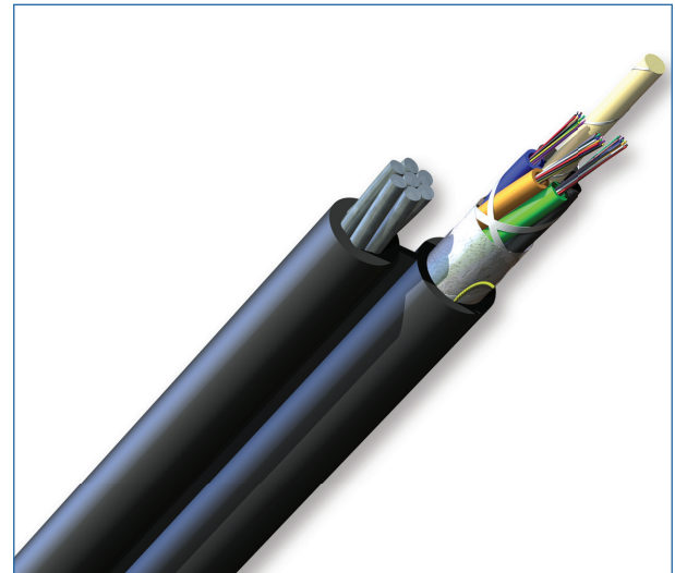
Part Number: 036TUA-T4131D20
