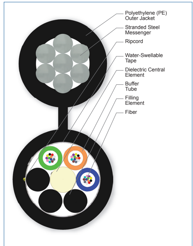
Cross Section of Part Number: 036TUA-T4131D20
