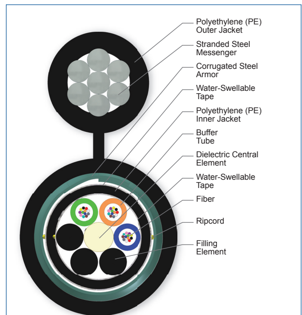
Cross Section of Part Number: 036TUB-T4131D20
