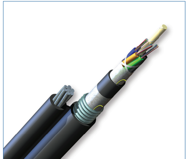
Part Number: 036TUB-T4131D20
