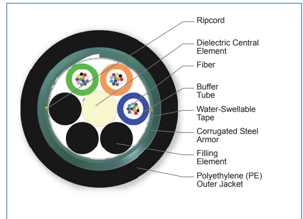
Cross Section of Part Number: 036TUC-T4180D20
