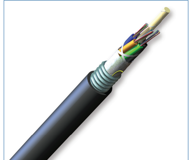
Part Number: 036TUC-T4180D20
