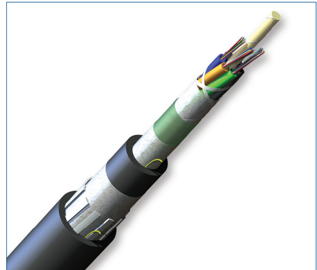
Part Number: 036TUL-T4680D2N
