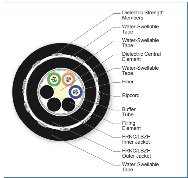
Cross Section of Part Number: 036TUL-T4680D2N
