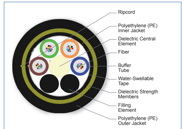
Cross Section of Part Number: 048EAE-T4501A20
