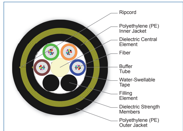
Cross Section of Part Number: 048EAE-T4A01A20
