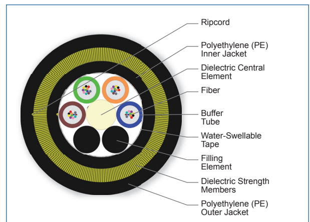
Cross Section of Part Number: 048EAE-T4E01A20
