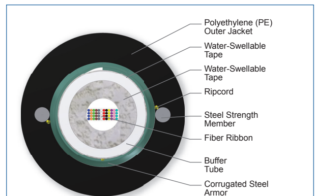
Cross Section of Part Number: 048EC5-14100D53
