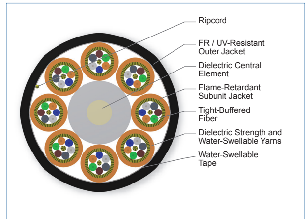
Cross Section of Part Number: 048K8F-61130-29
