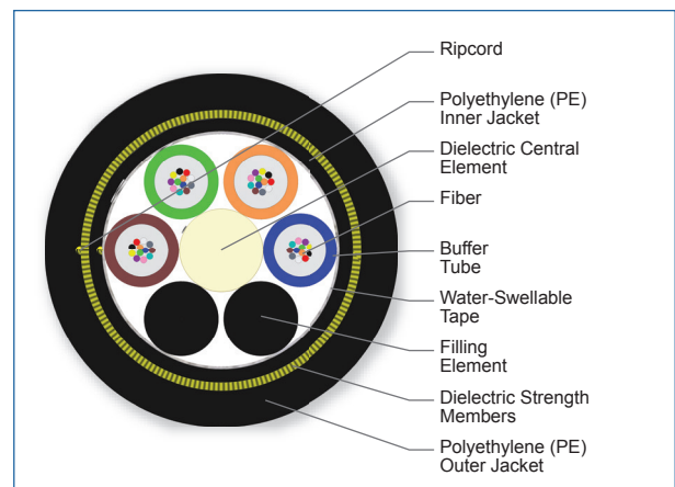
Cross Section of Part Number: 048KAE-T4230A20
