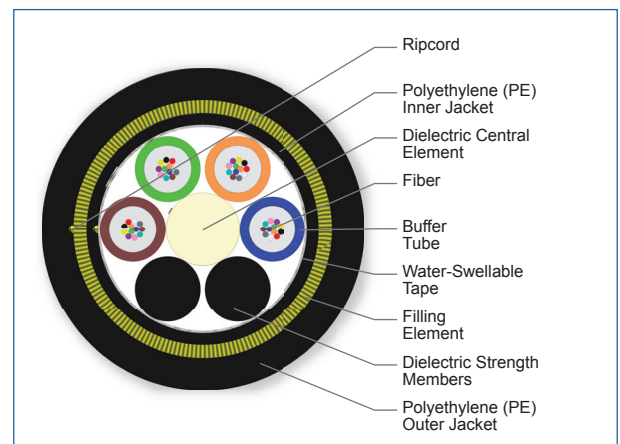
Cross Section of Part Number: 048KAE-T4530A20
