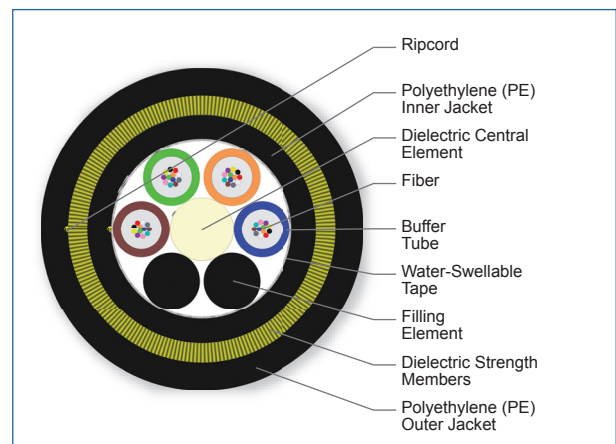
Cross Section of Part Number: 048KAE-T4A30A20
