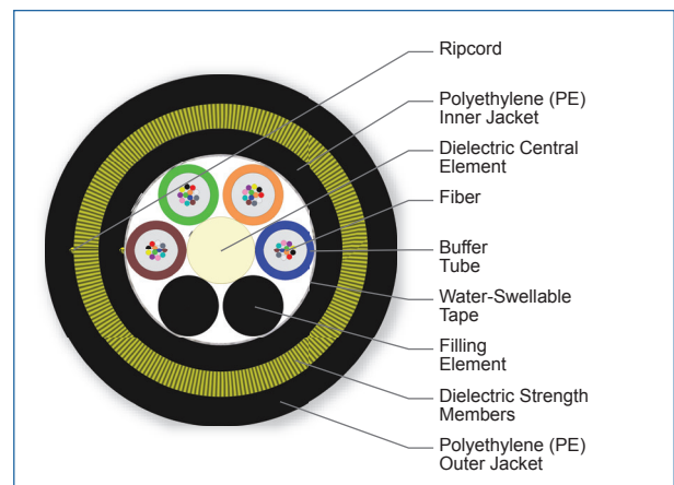
Cross Section of Part Number: 048KAE-T4C30A20
