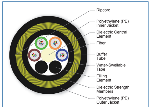
Cross Section of Part Number: 048KAE-T4E30A20
