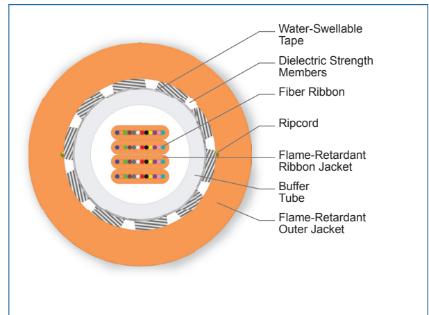
Cross Section of Part Number: 048KC8-94130-20
