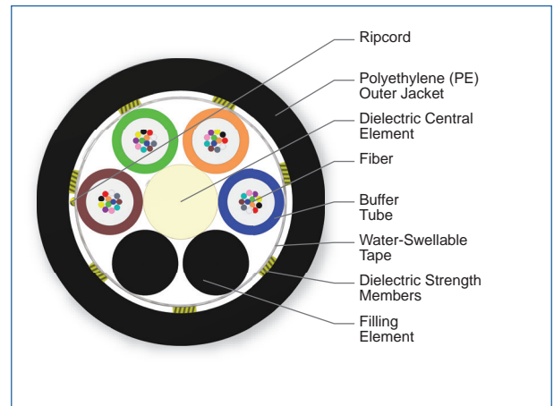
Cross Section of Part Number: 048KN4-T4M30A20
