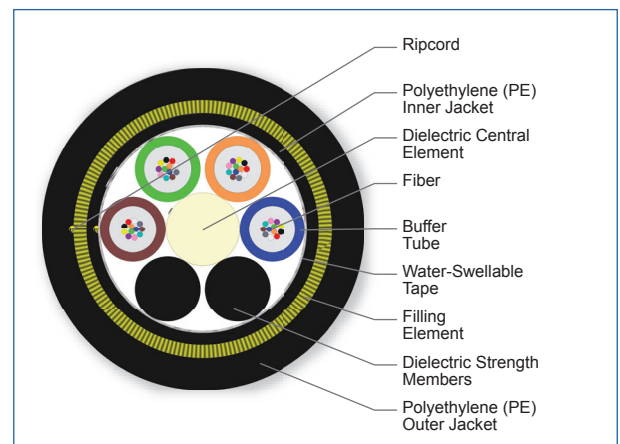
Cross Section of Part Number: 048TAE-T4531A20
