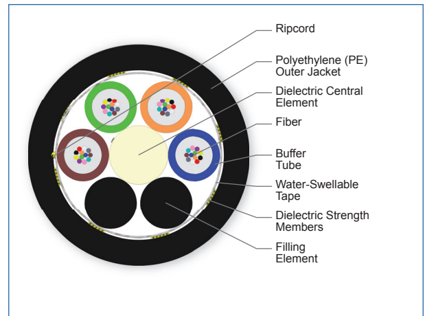
Cross Section of Part Number: 048TN4-T4S31A20
