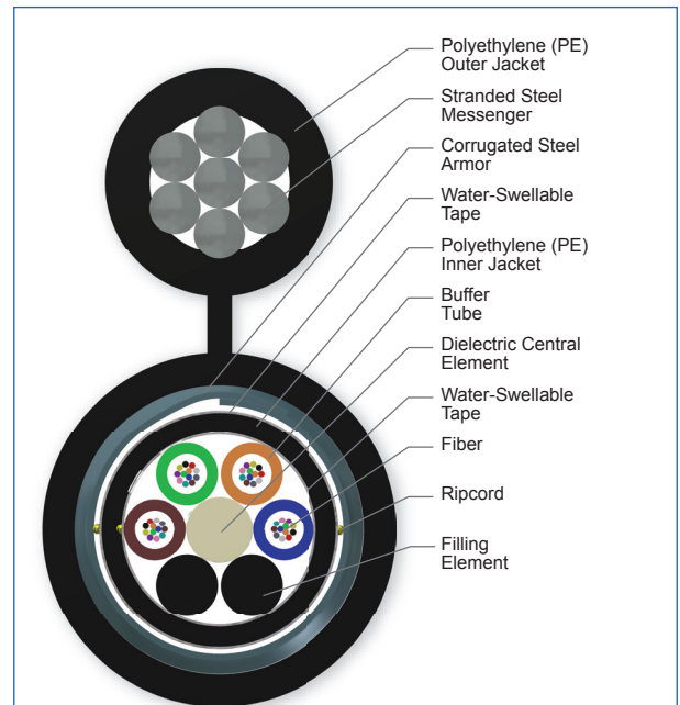
Cross Section of Part Number: 048TUB-T4131D20
