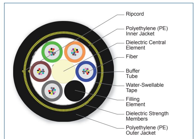
Cross Section of Part Number: 060EAE-T4201A20
