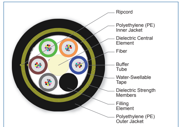
Cross Section of Part Number: 060EAE-T4501A20
