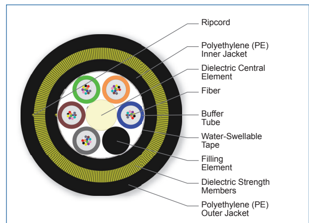
Cross Section of Part Number: 060EAE-T4C01A20
