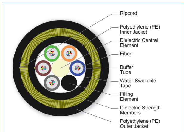
Cross Section of Part Number: 060EAE-T4E01A20
