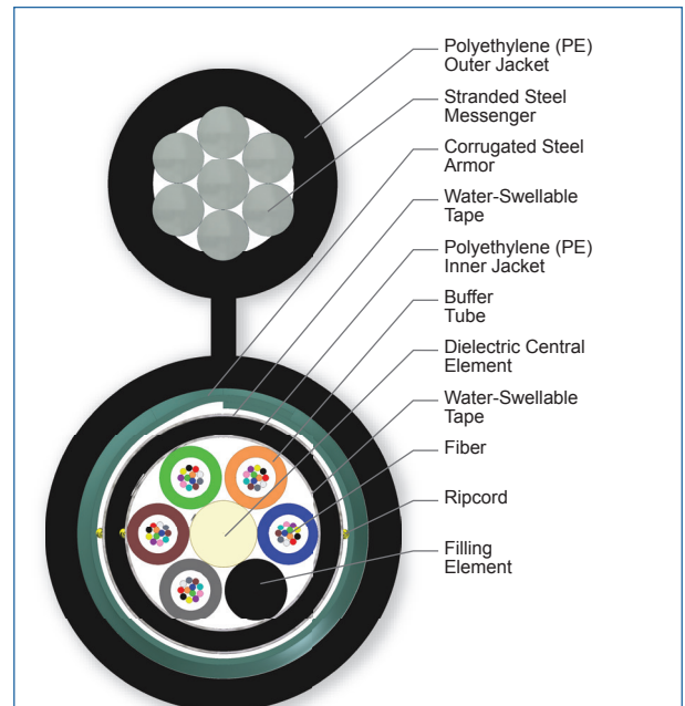
Cross Section of Part Number: 060EUB-T4101D20
