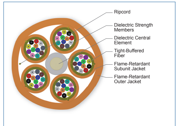
Cross Section of Part Number: 060K81-T3130-24
